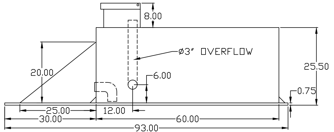
SIDE VIEW
