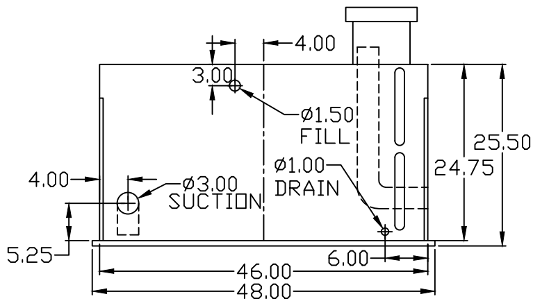
REAR VIEW
